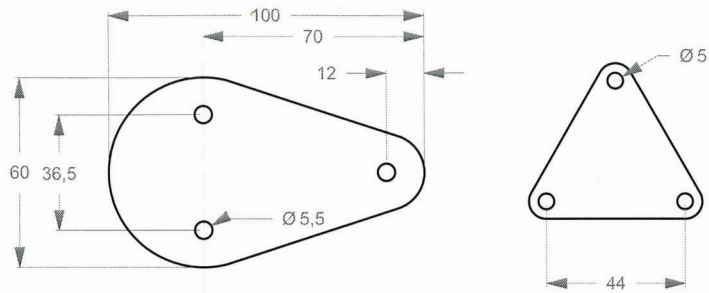
Montagegaten beugels / Mounting holes bracket
